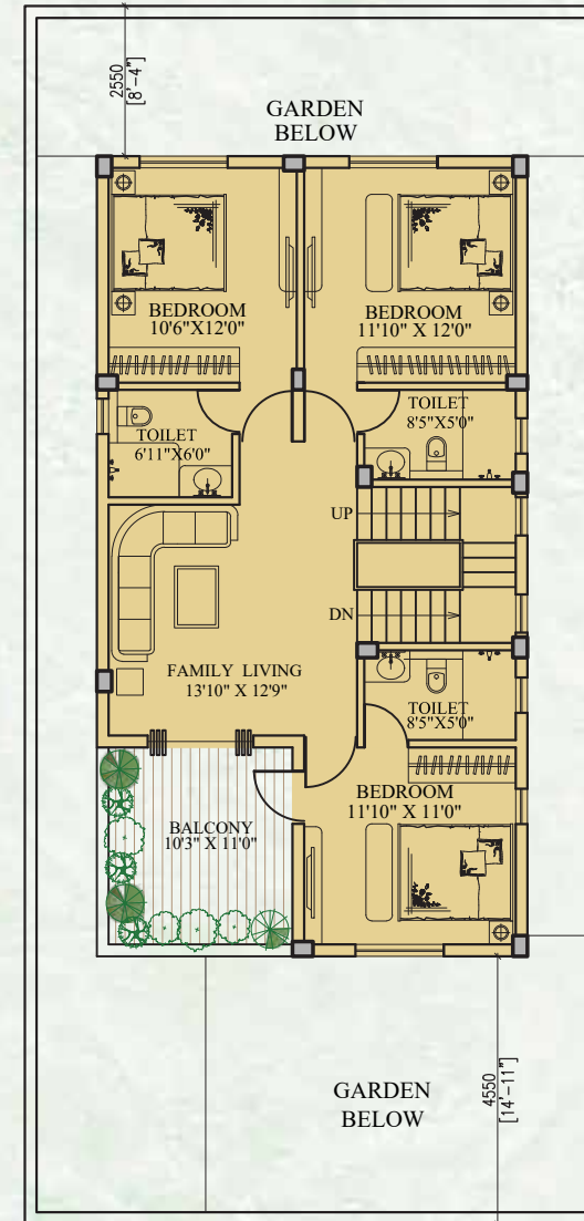
FIRST FLOOR AREA - 1072 Sq.Ft.
